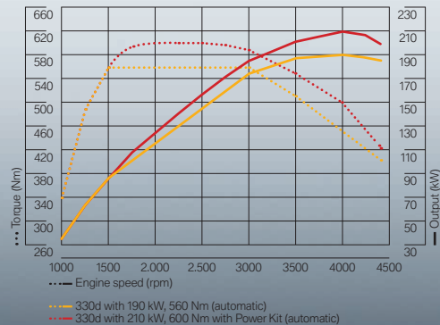
Data for the BMW 330d with BMW M Performance Power Kit 330d under full load
